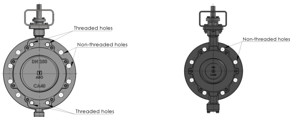
Fig. 15: Connection design for valves with DF (Double flange) type body
