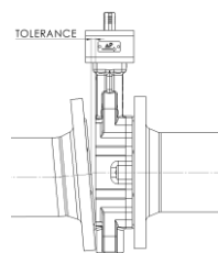
Fig. 4: Parallelism of flanges
